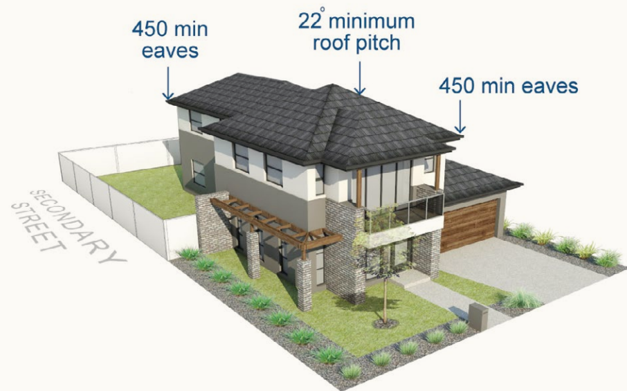
Diagram 03: Roof Design
